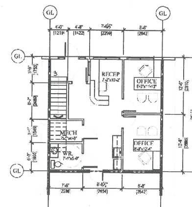
OPTION A MAIN FLOOR OFFICE LAYOUT SCALE: 1/8"=1'-0"
