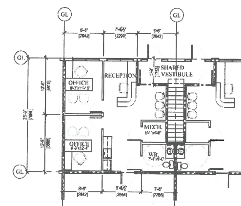
OPTION B MAIN FLOOR OFFICE LAYOUT SCALE: 1/8"=1'-0"
